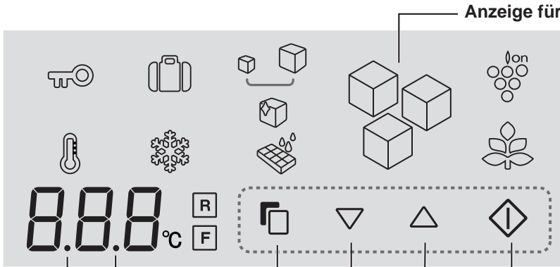
Tasten
